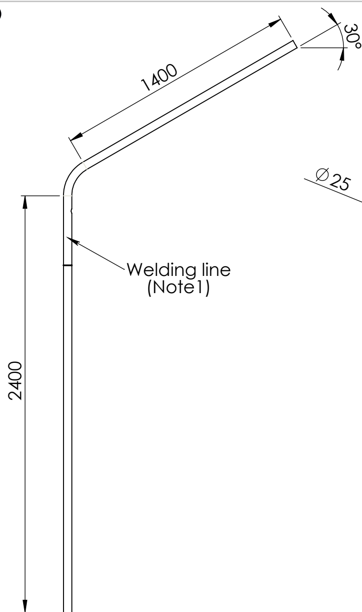
DETAIL N SCALE 1 : 5
