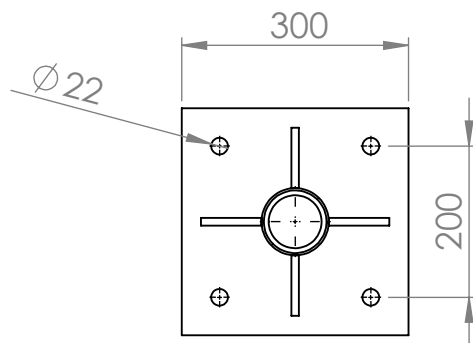
SECTION J-J Base plate Thickness: 10mm
