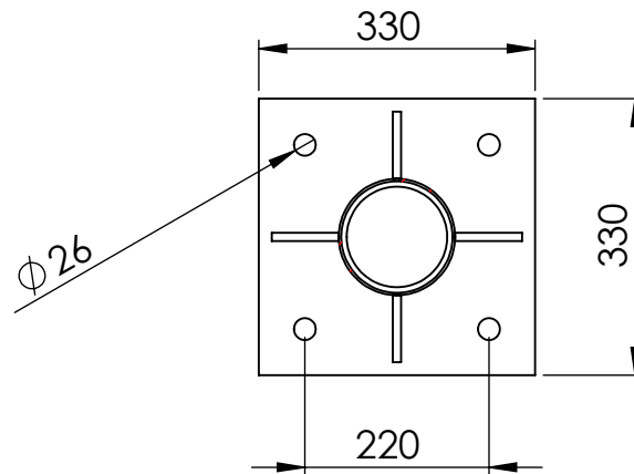
SECTION X-X Base plate- Th: 15 mm
