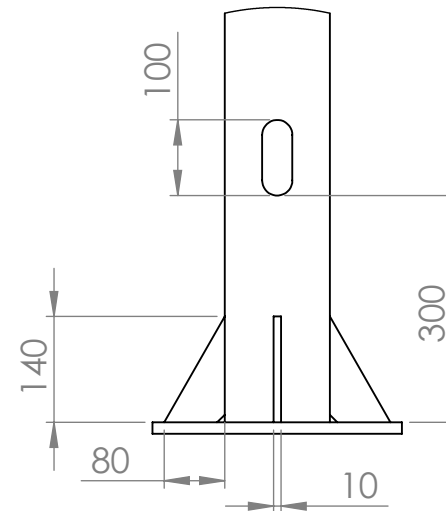
DETAIL U SCALE 1 : 10
