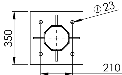
SECTION B-B Base plate Th: 15 mm
